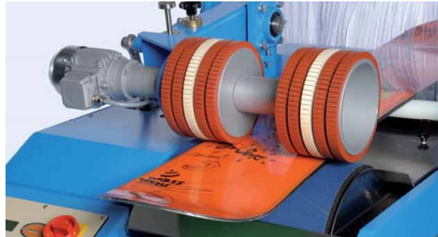
Splitable drive roll for perfect pressure distribution for convex and concave Snowboard shape
