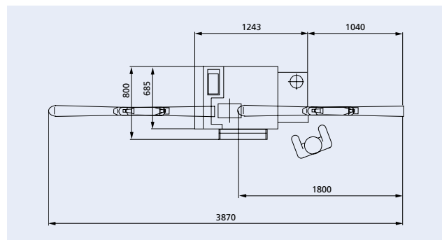
Layout PROFI S150
